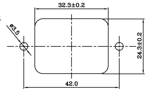
PANEL CUT-OUT
